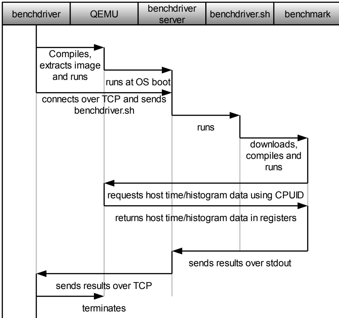
Figure 13: Interaction between processes involved in measuring performance.
