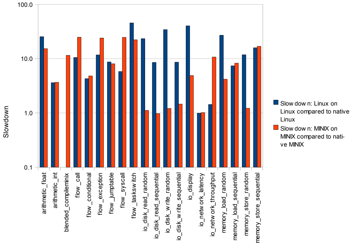
Figure 15: Slow-down caused by emulation
