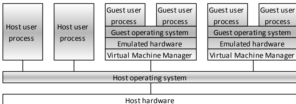
Figure 2: The virtual machine manager as a regular user process
