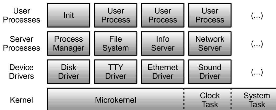
Figure 1: Structure of the MINIX 3 operating system, each box denoting a process isolated from the other processes; source: [21].
