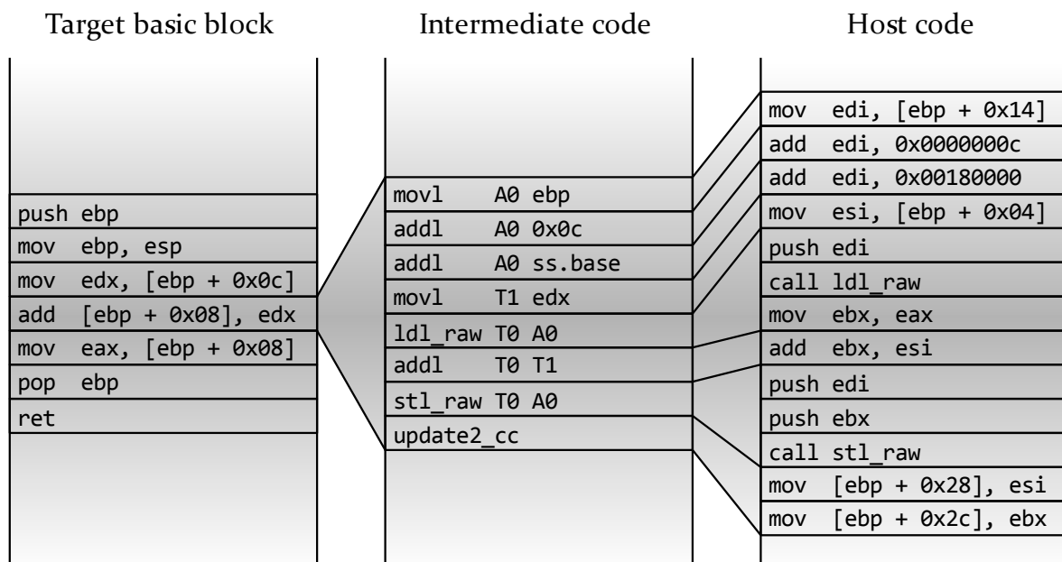
Figure 9: Translation of a x86 function using intermediate code
