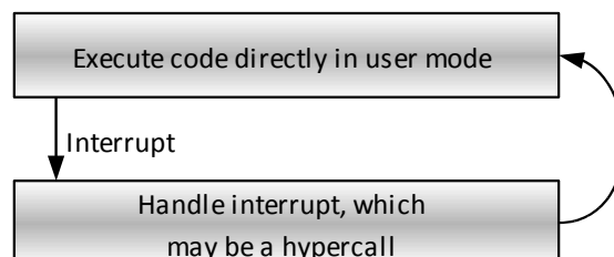
Figure 4: Main loop for paravirtualization
