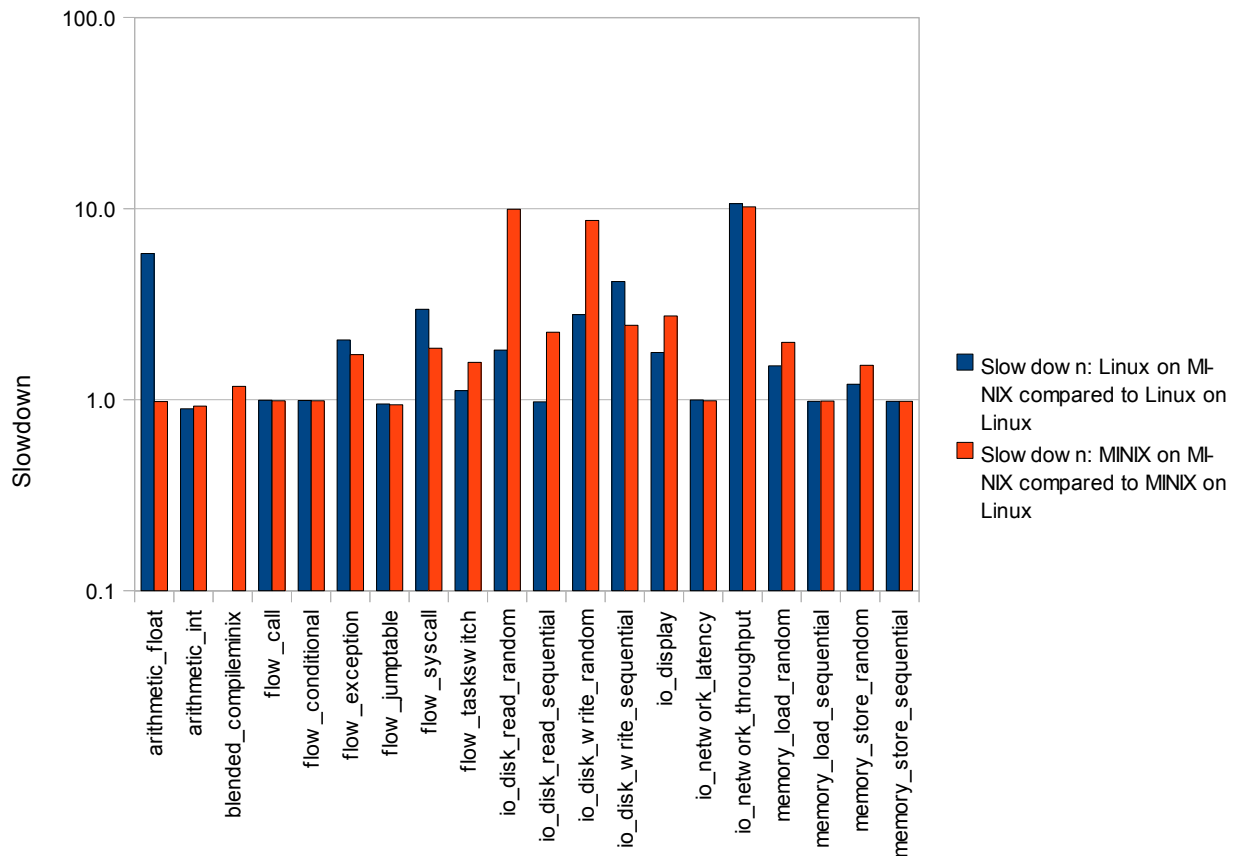
Figure 17: MINIX vs. Linux as a host platform
