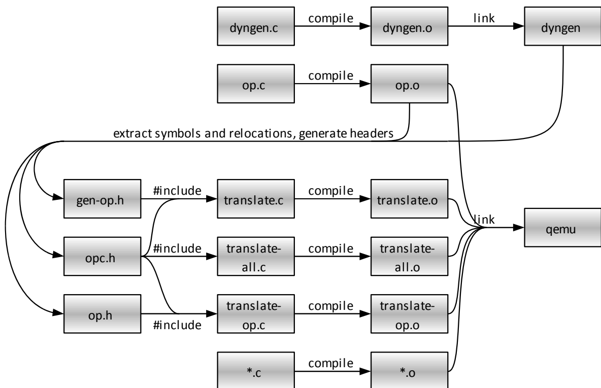
Figure 8: Steps in the compilation of QEMU using the Dyngen tool
