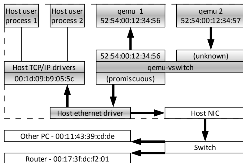
Figure 11: qemu-vswitch routing an outgoing DHCP discover packet
