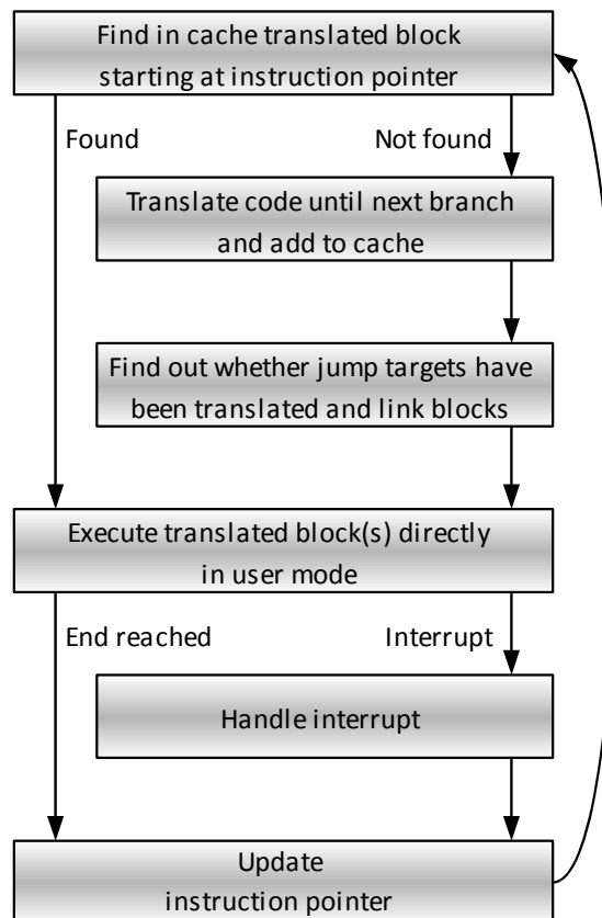
Figure 3: Main loop for binary dynamic translation
