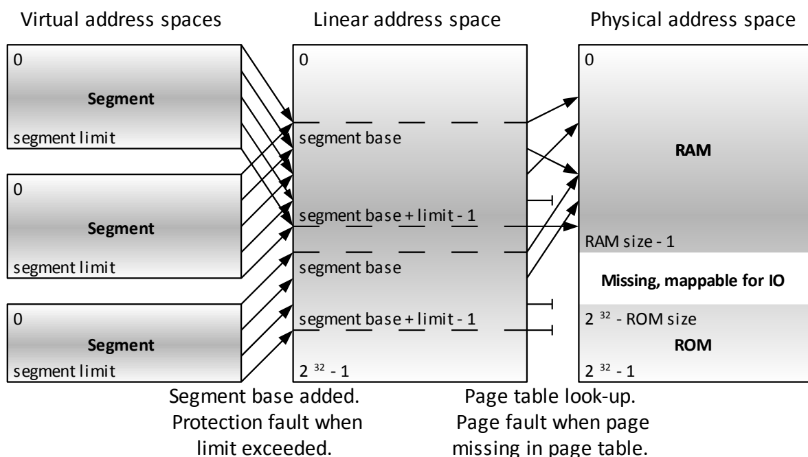
Figure 6: MMU operation and terminology on x86
