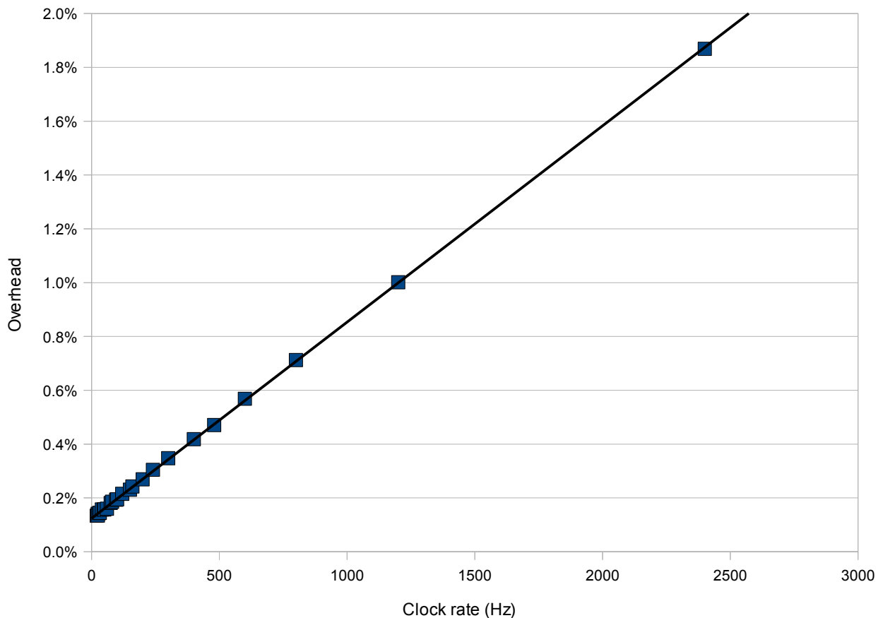
Figure 19: Relationship between overhead caused by the operating system and timer frequency, on MINIX patched to have a variable clock frequency
