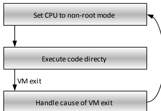
Figure 5: Main loop for hardware-supported virtualization
