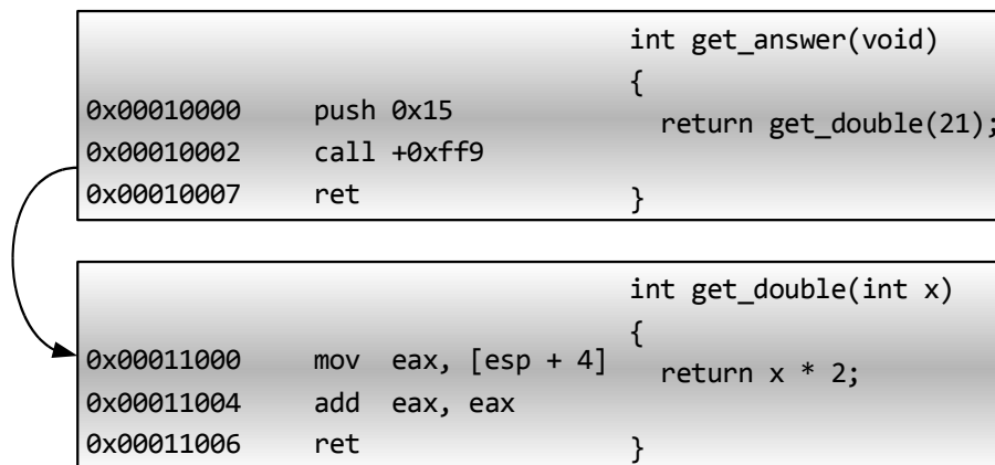
Figure 7: Function call with relative displacement on x86
