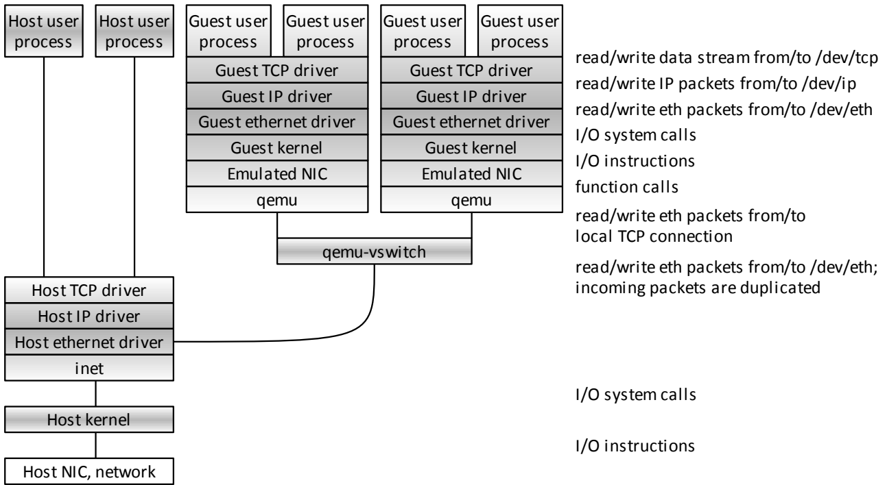
Figure 10: Processes involved in network emulation using qemu-vswitch
