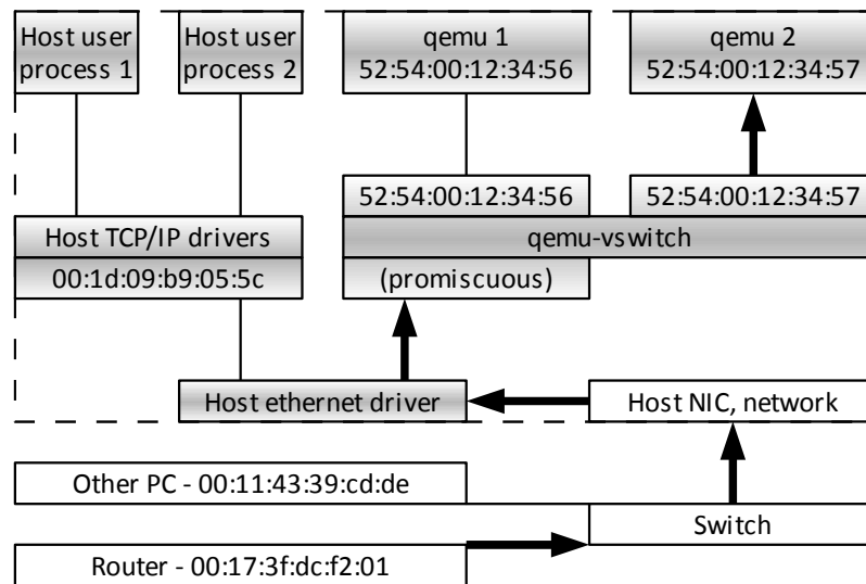
Figure 12: qemu-vswitch routing an incoming DHCP offer packet
