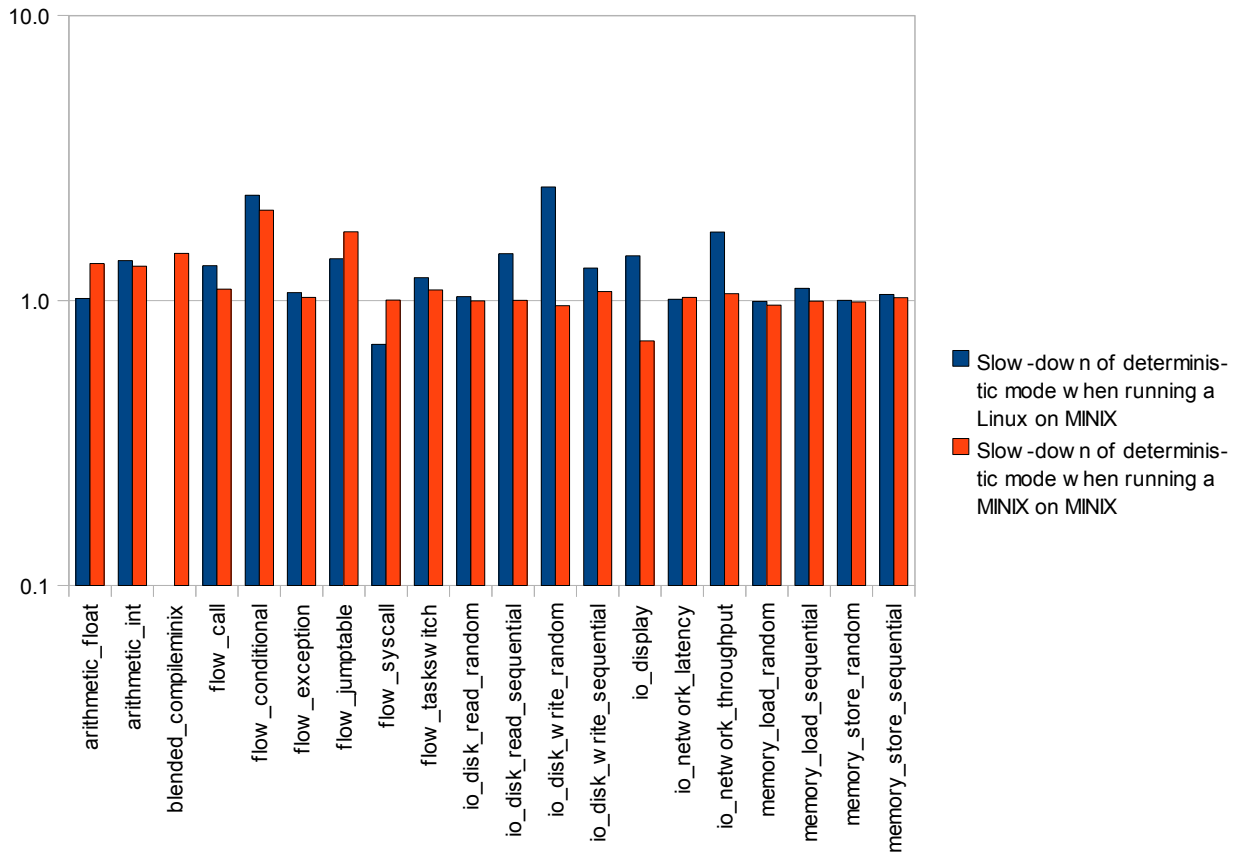
Figure 18: Slow-down of deterministic mode compared to default mode on MINIX
