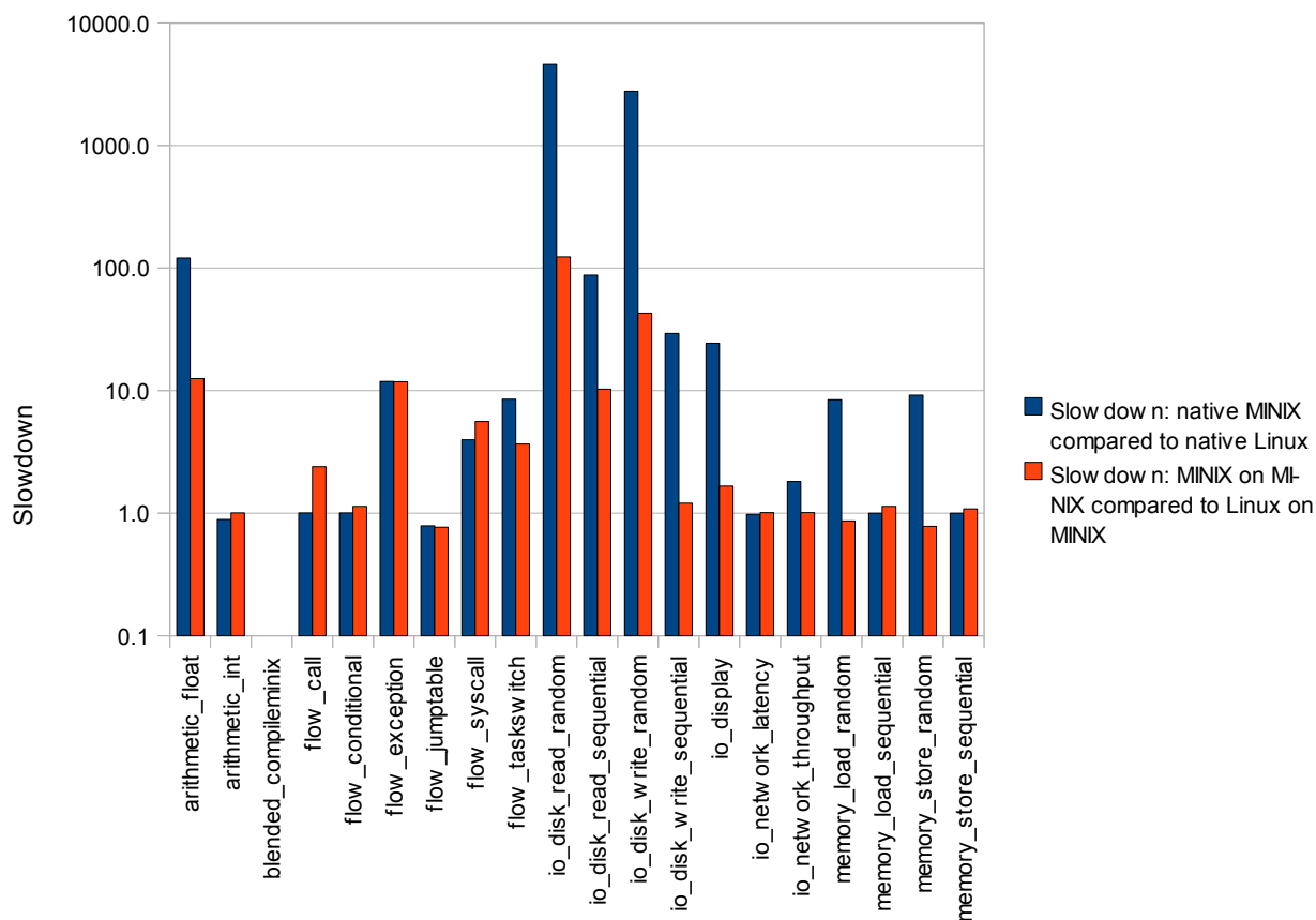
Figure 14: MINIX vs. Linux as a guest platform
