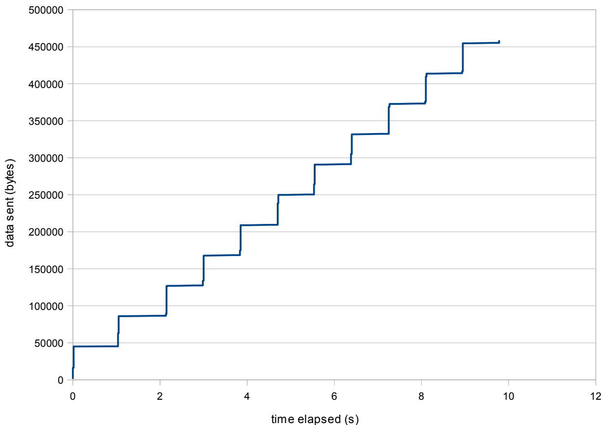
Figure 16: Amount of data sent in the io_network_throughput benchmark
